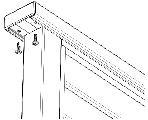
3) Fix end cap to undercapping rail (** refer text above if installing a white balustrade)
