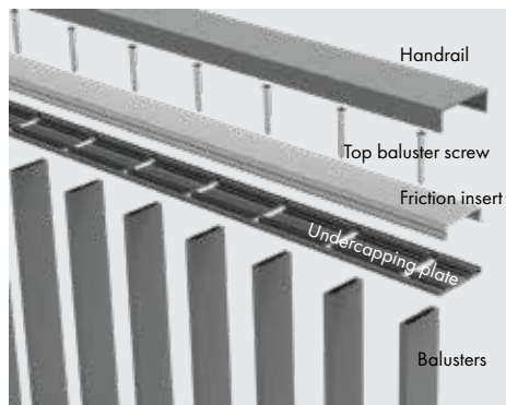
EXPLODED VIEW
