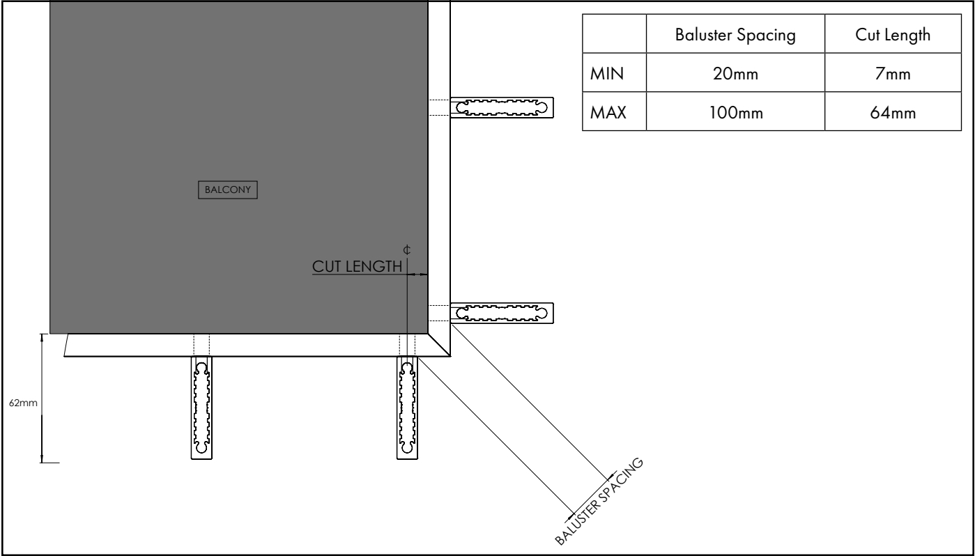
● Option 1: External Corners
