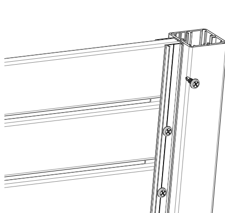
2) Fix off horizontal slats through side frame
