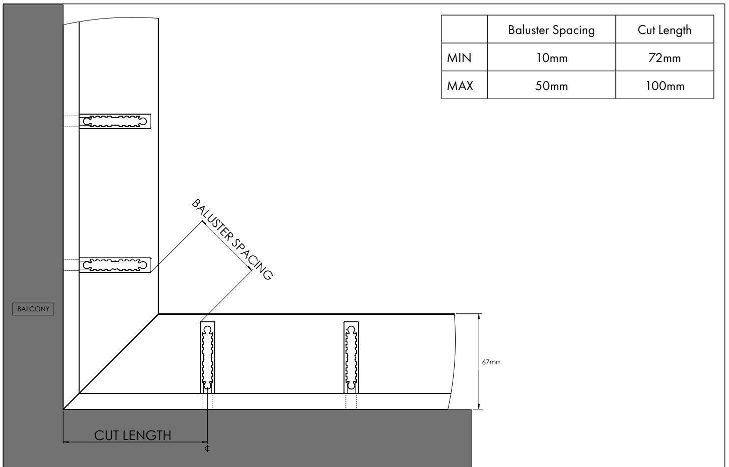
● Option 2: Internal Corners
