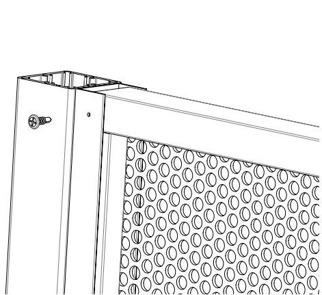
3) Fixes together framing kit vertical sides and U channel
