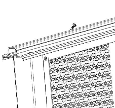
4) Fixes undercapping rail to framing kit
