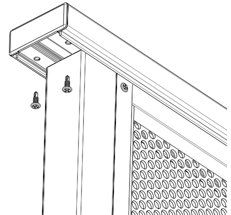
5) Fixes end cap to undercapping rail
